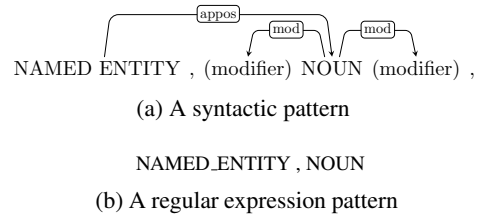
Figure 1: Patterns capturing appositions
