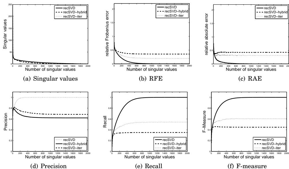
Fig. 6: FLICKR dataset. Performance of the RecSVD, Iterative and Hybrid algorithms as a function of the number of singular values; x -axis: number of singular values; y -axis: magnitude of the singular values (2(a)), RFE (2(b)), RAE (2(c)), Precision (2(d)), Recall (2(e)), F-measure (2(f)).
