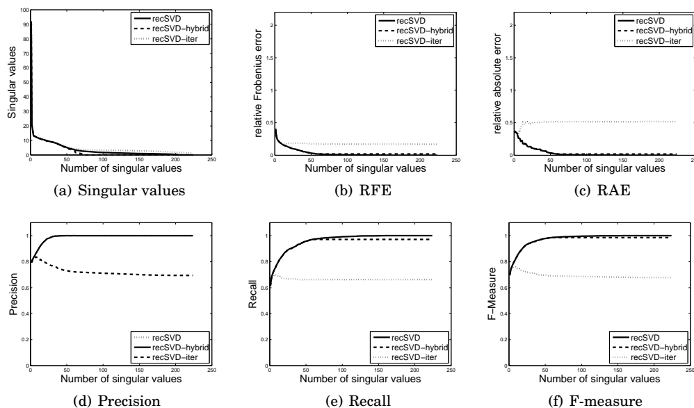
Fig. 4: MP3 dataset. Performance of the RecSVD, Iterative and Hybrid algorithms as a function of the number of singular values; x -axis: number of singular values; y -axis: magnitude of the singular values (4(a)), RFE (4(b)), RAE (4(c)), Precision (4(d)), Recall (4(e)), F-measure (4(f)).
