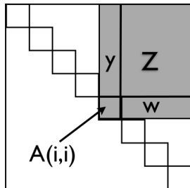
Fig. 1: The mechanics of the LS algorithm for reconstructing the main diagonal elements of L and R .
