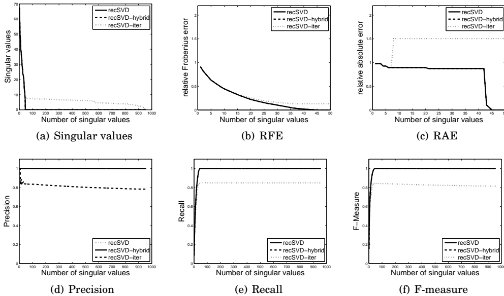
Fig. 2: Performance of the RecSVD, Iterative and Hybrid algorithms on the BLOCK dataset; x -axis: number of singular values; y -axis: singular values ( 2(a)), RFE ( 2(b)), RAE ( 2(c)), Precision ( 2(d)), Recall ( 2(e)), F-measure ( 2(f)).
